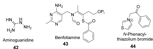
Scheme 8. Structures of AGE inhibitors and “AGE breakers”.
